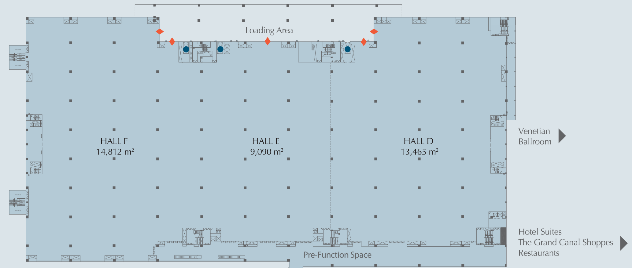
Cotai Strip® CotaiExpo™ Level Three – Total 37,367 m 2
